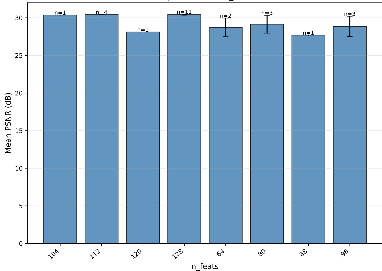
Mean PSNR per value of n_feats — SwinT
